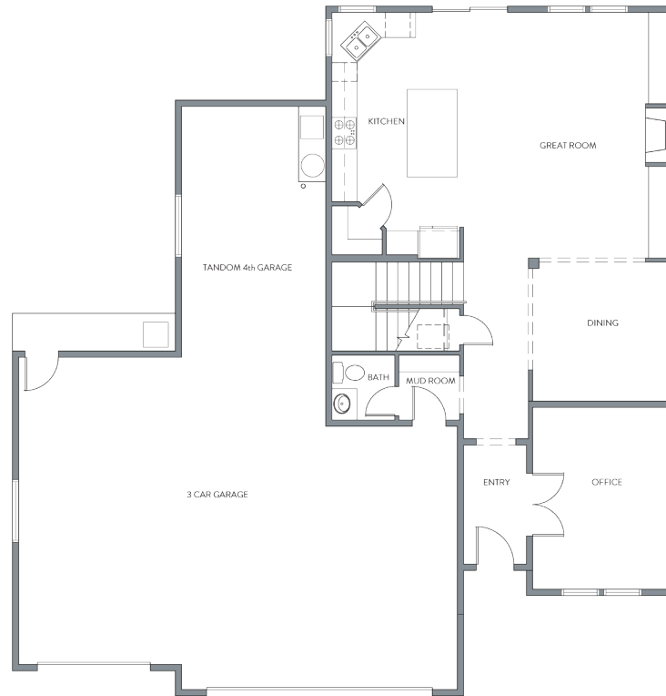
STORY 1
